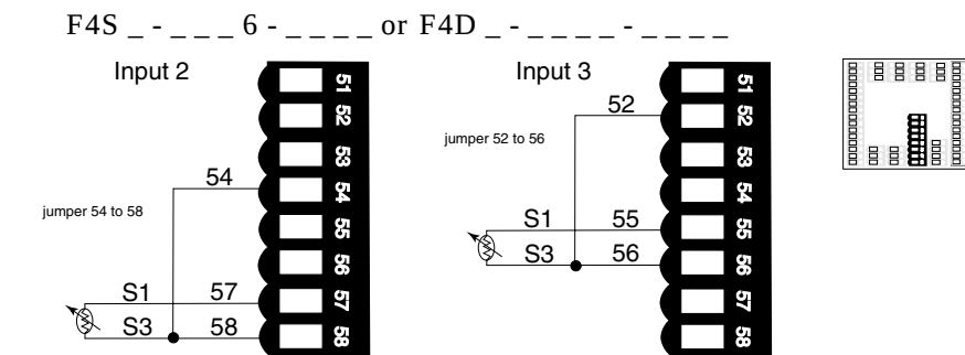
Figure 12.4b — RTD (2-wire) 100Ω Platinum
