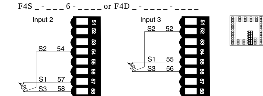
Figure 12.4c — RTD (3-wire) 100Ω Platinum
